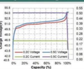
Charge Characteristics @ 0.2C 25°C
