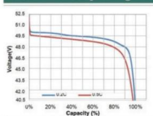
Different Rate Discharge Curve @ 25°C
