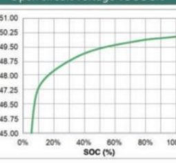
Open circuit voltage VS SOC%
